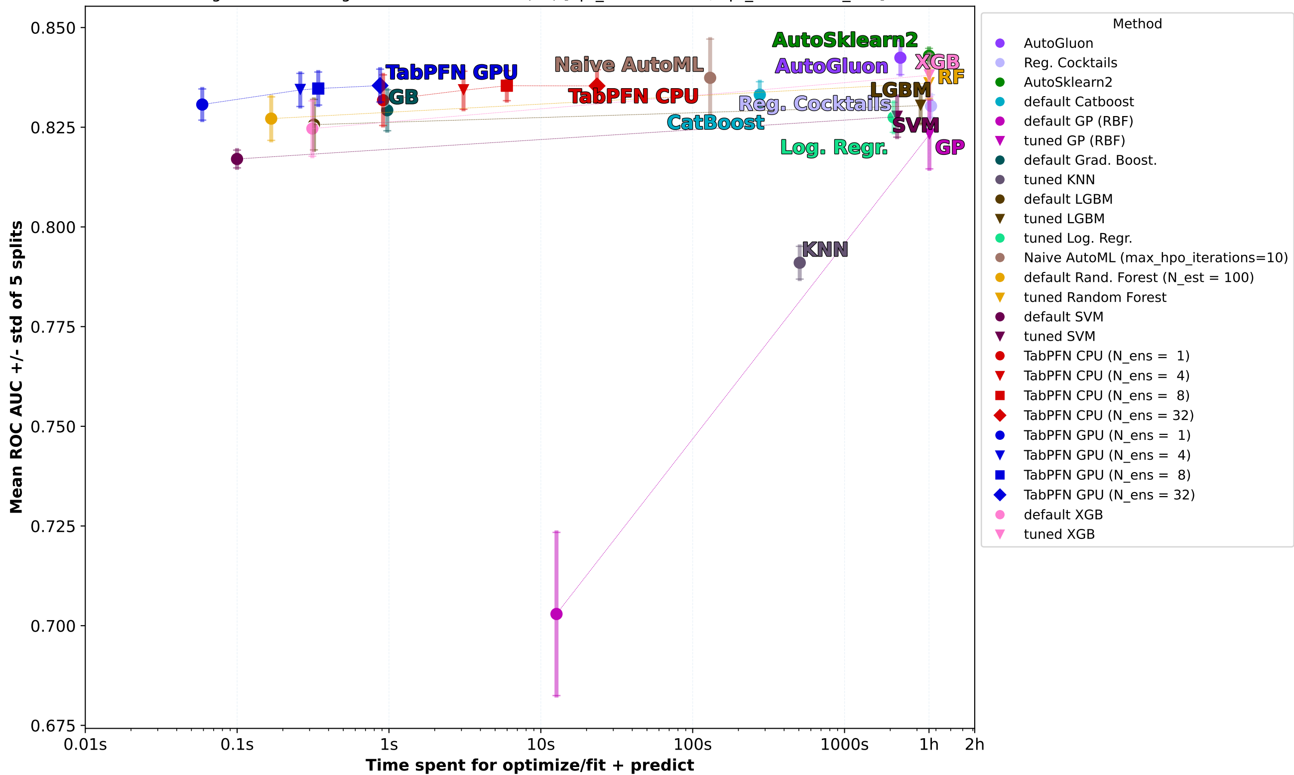
Categorical or Missing Values Test Datasets (12) [opt_time=3600.0, opt_metric=roc_auc]
