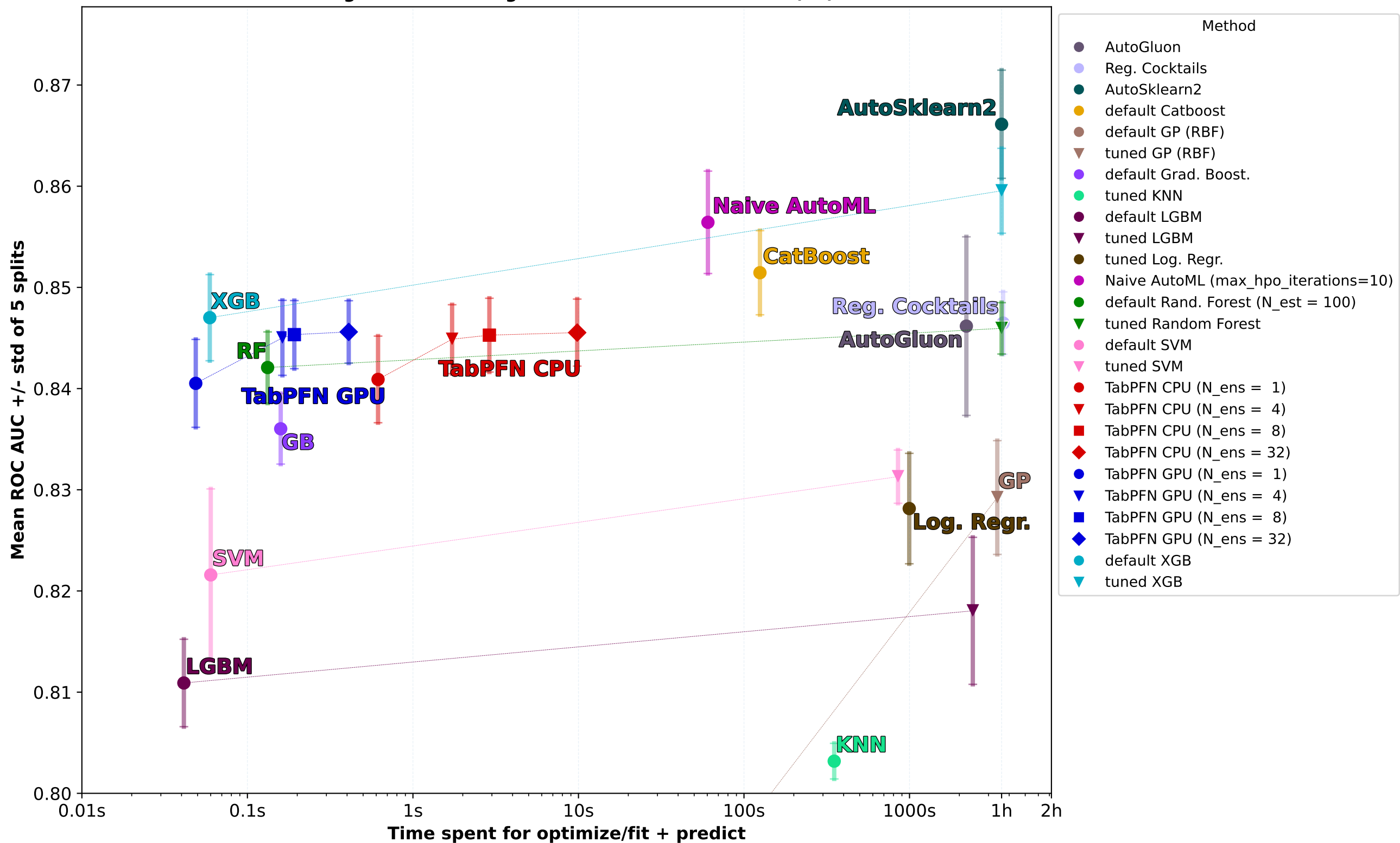
Categorical or Missing Values Validation Datasets (84)
