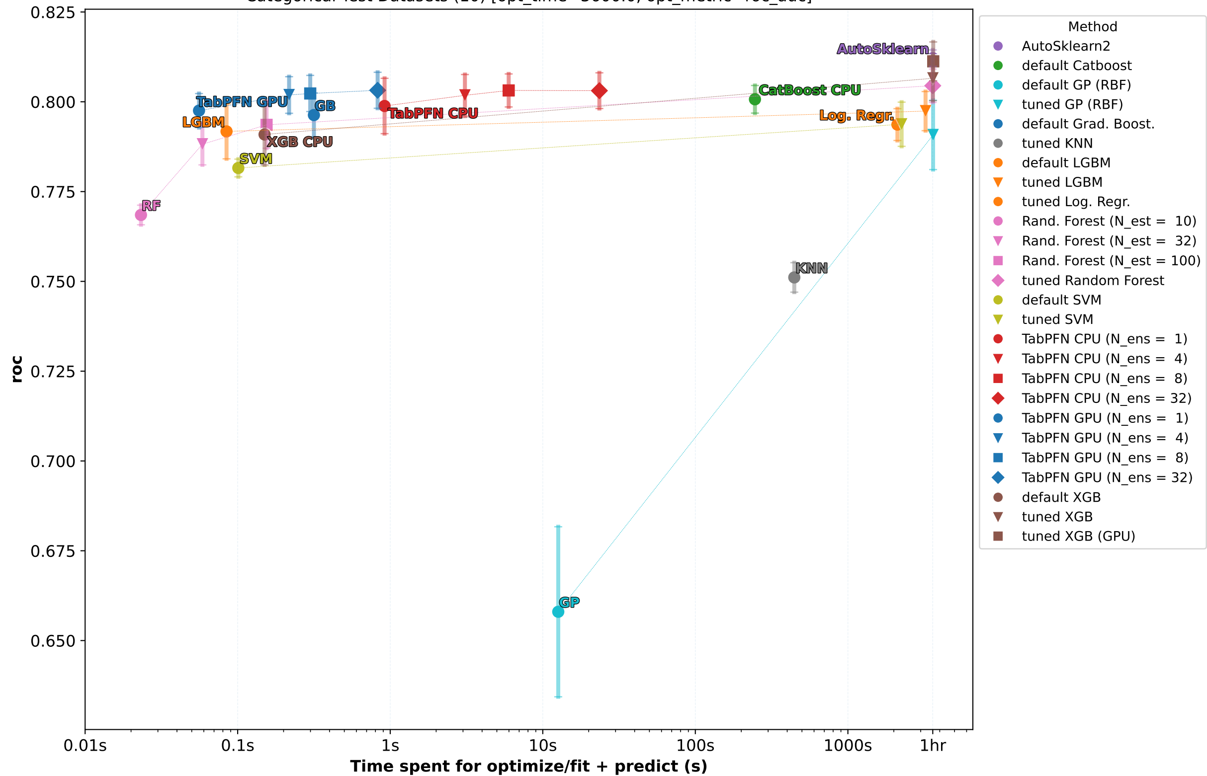
Categorical Test Datasets (10) [opt_time=3600.0, opt_metric=roc_auc]
