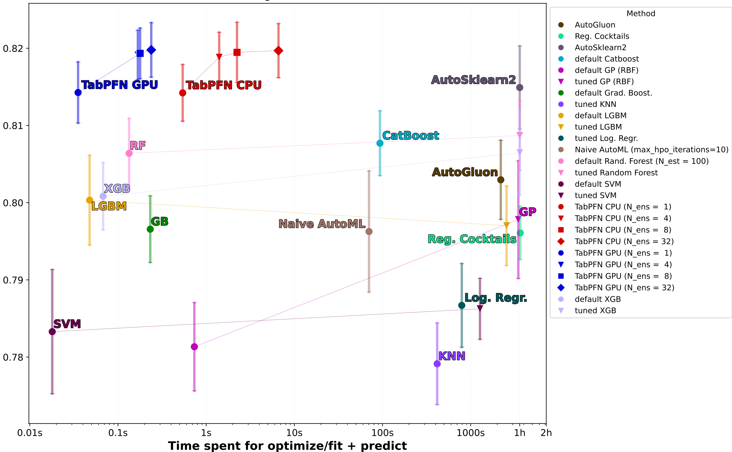
Numerical and No Missing Values Validation Datadets (65)
