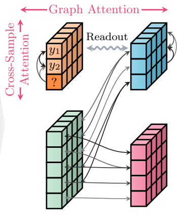
(c) Reason across Tables
