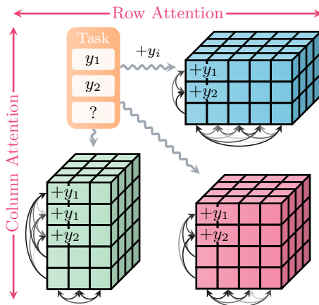
(b) Reason within Tables
