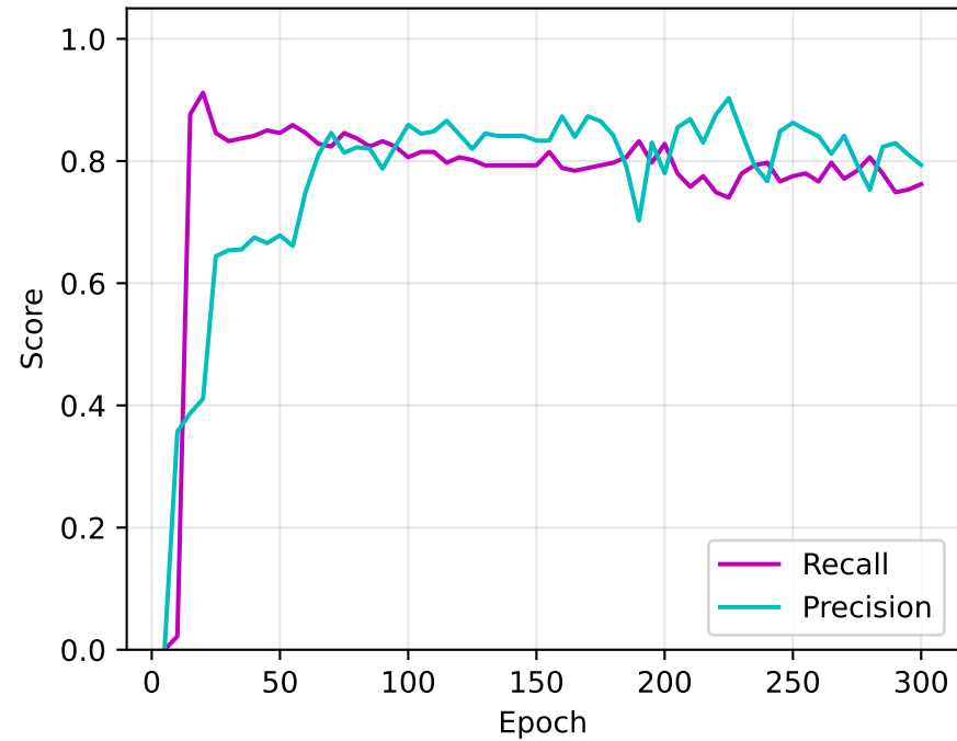
(c) Recall & Precision
