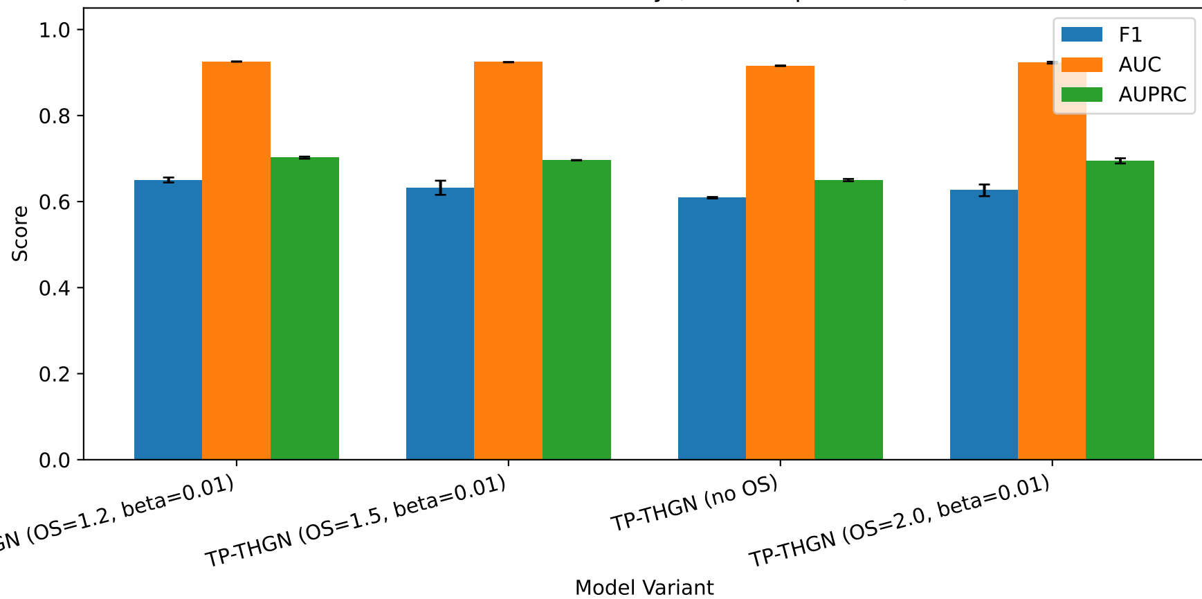
TP-THGN Ablation Study (Oversample Ratio)
