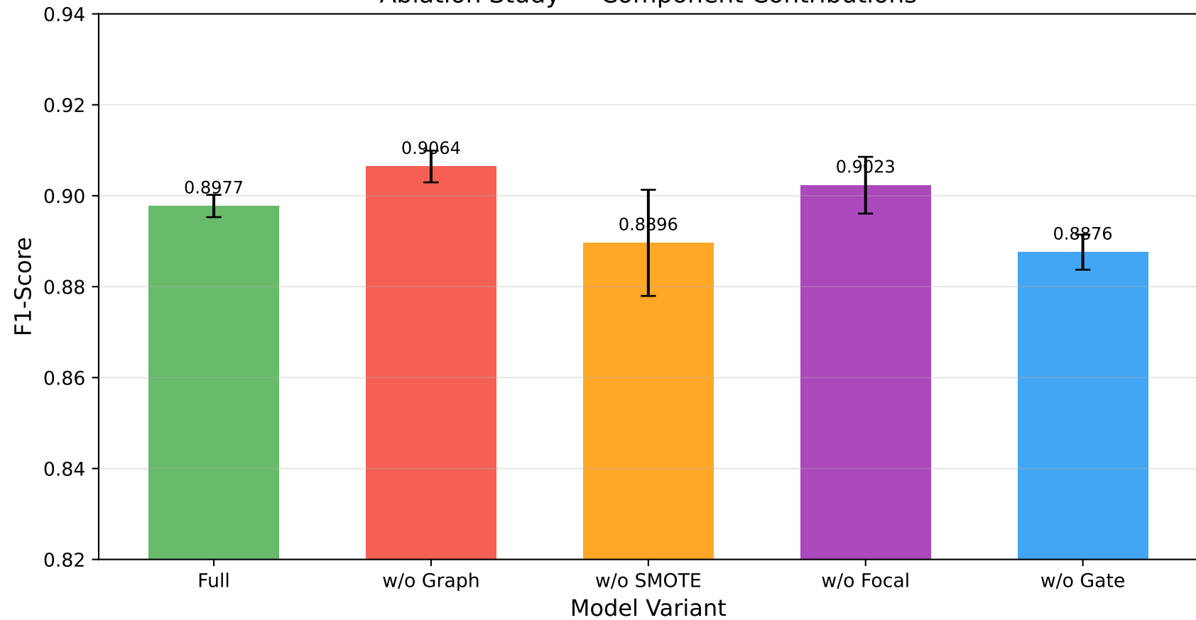
Ablation Study — Component Contributions
