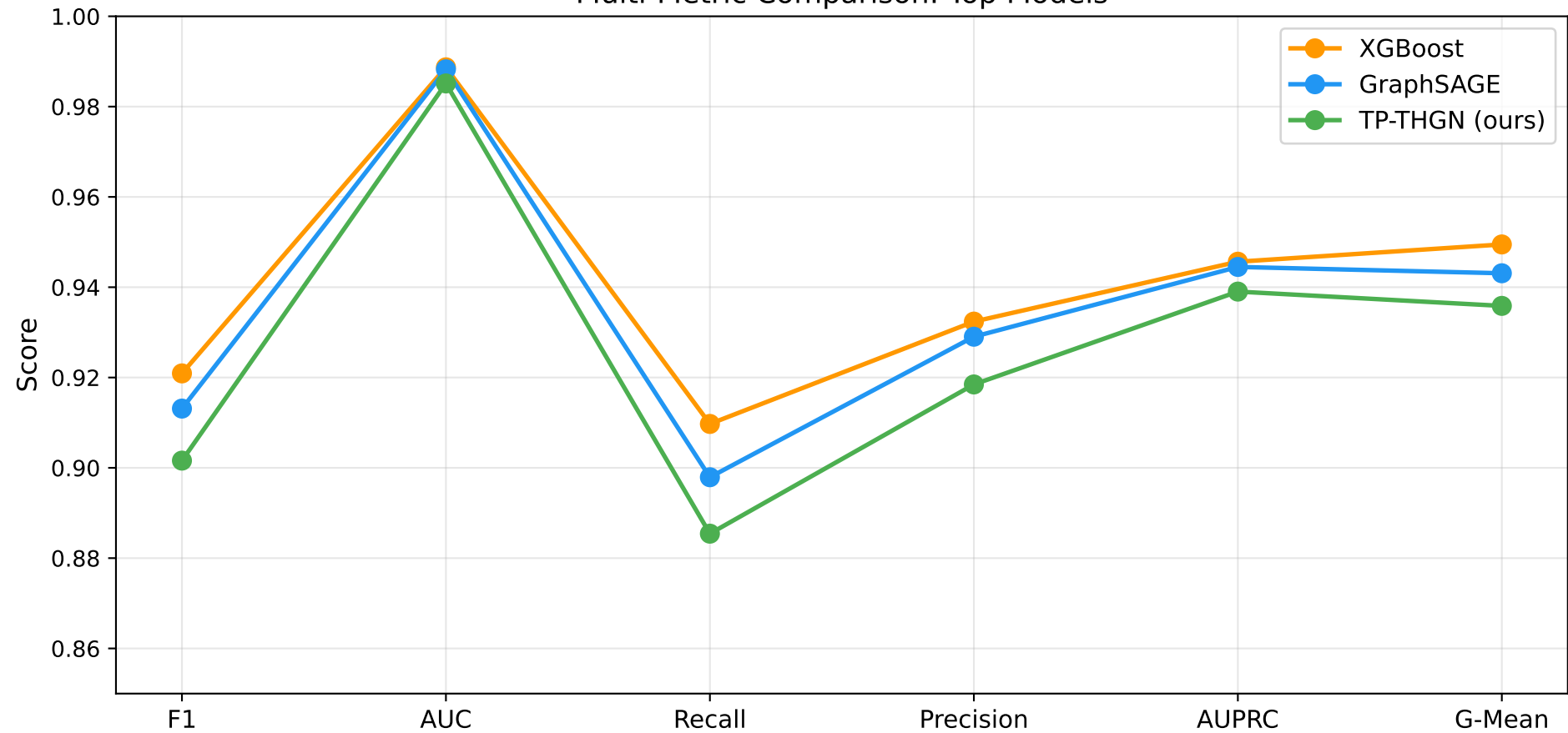
Multi-Metric Comparison: Top Models
