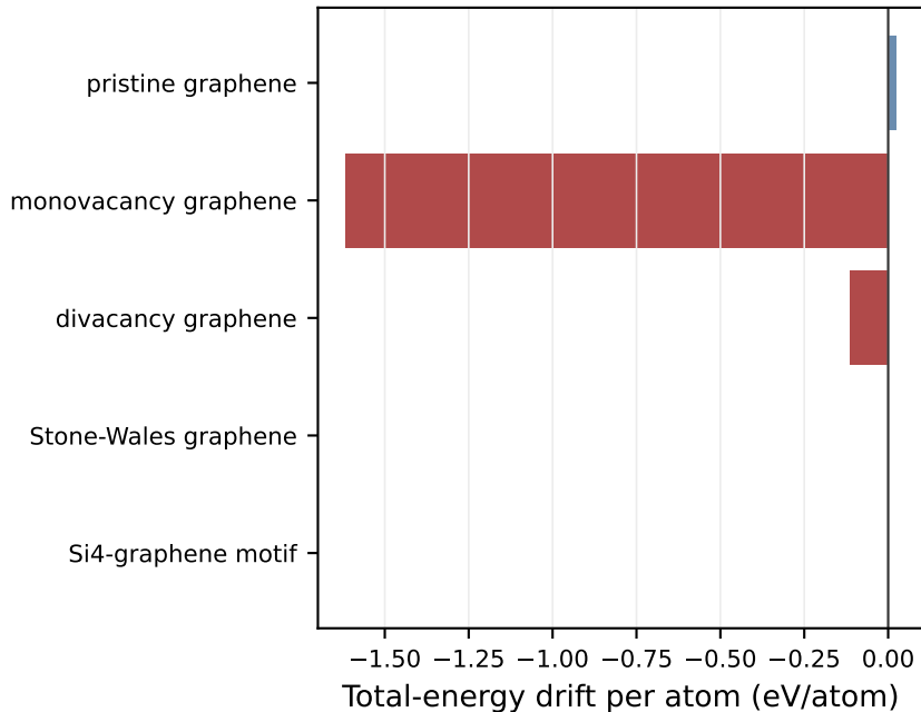
400 K NVT energy-drift diagnostic
