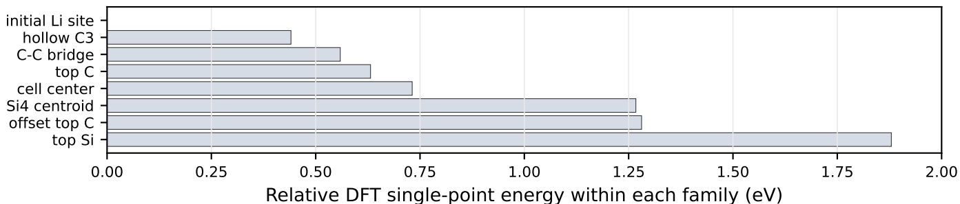
Si4-graphene motif
