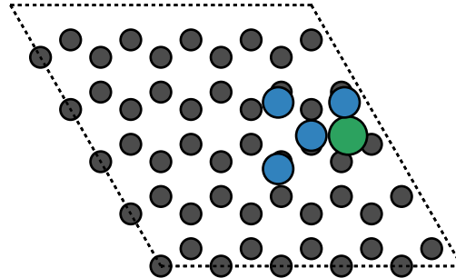
D_SiGraphene Si-graphene + Li
