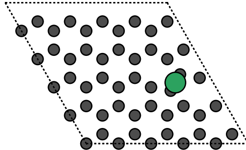
C_StoneWales Stone-Wales + Li
