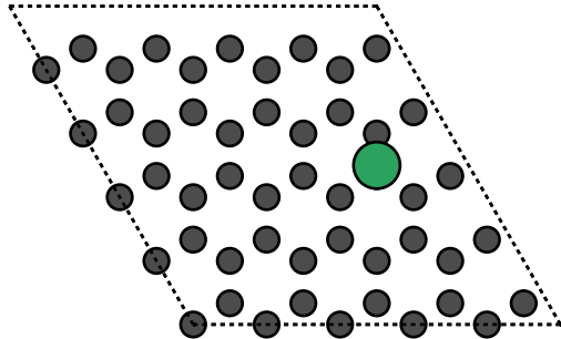
A_Perfect Pristine graphene + Li
