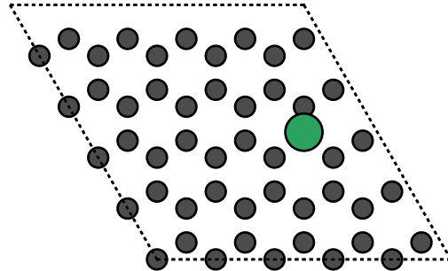
B1_Monovacancy Monovacancy + Li
