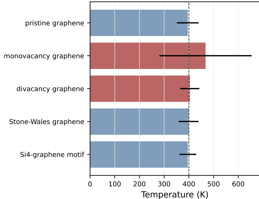
400 K NVT temperature diagnostic
