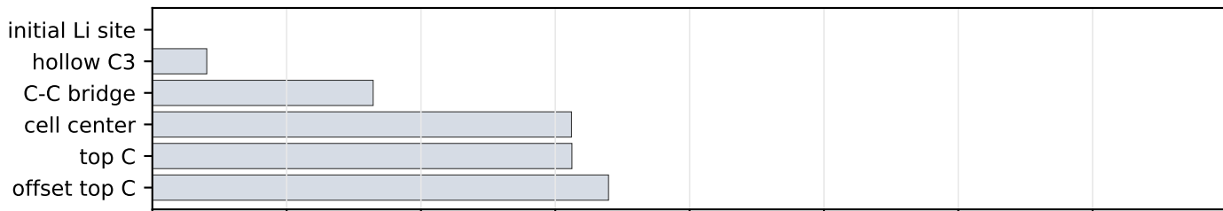
Stone-Wales graphene
