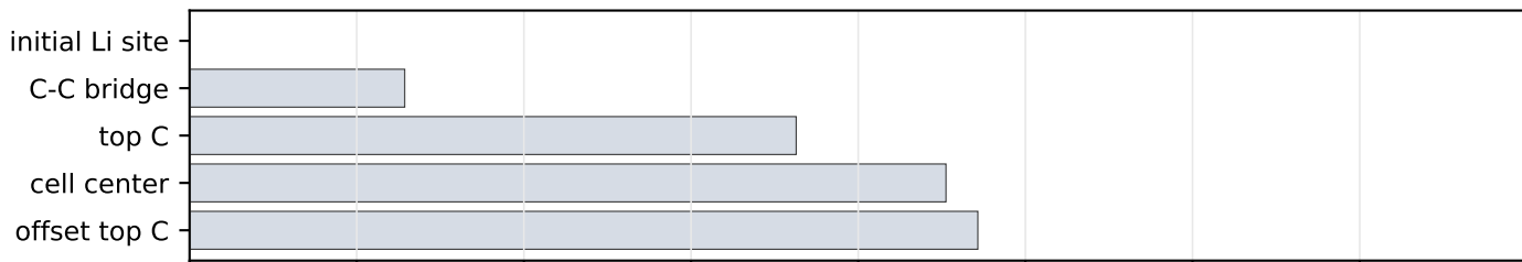
monovacancy graphene
