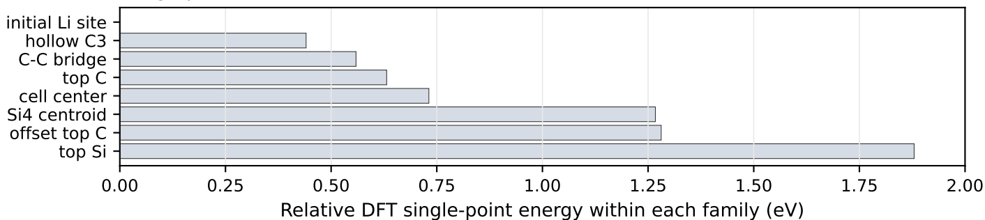
Si4-graphene motif
