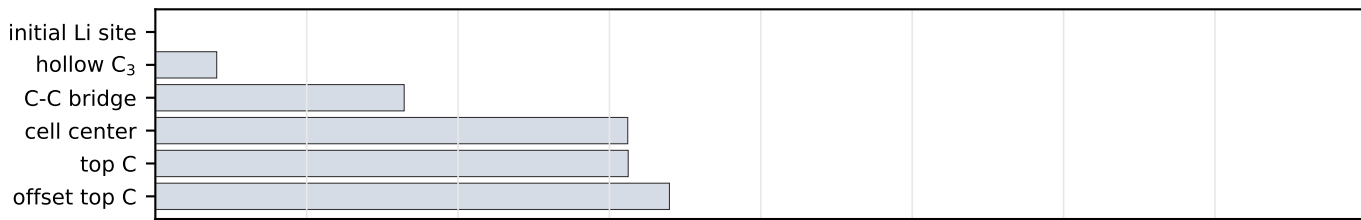
divacancy graphene
