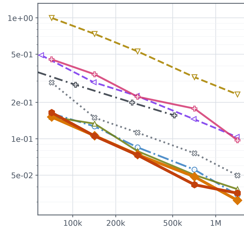
(c) Wine
