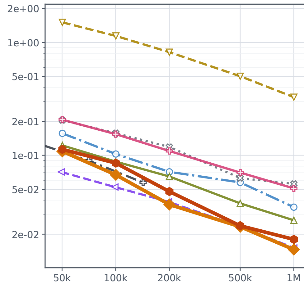
(b) Airport
