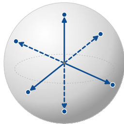
Balanced directions
