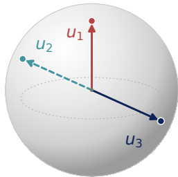
Center + normalize
