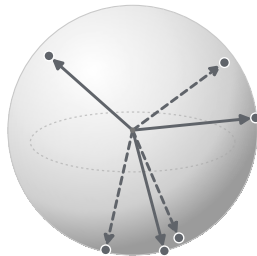
Random directions
