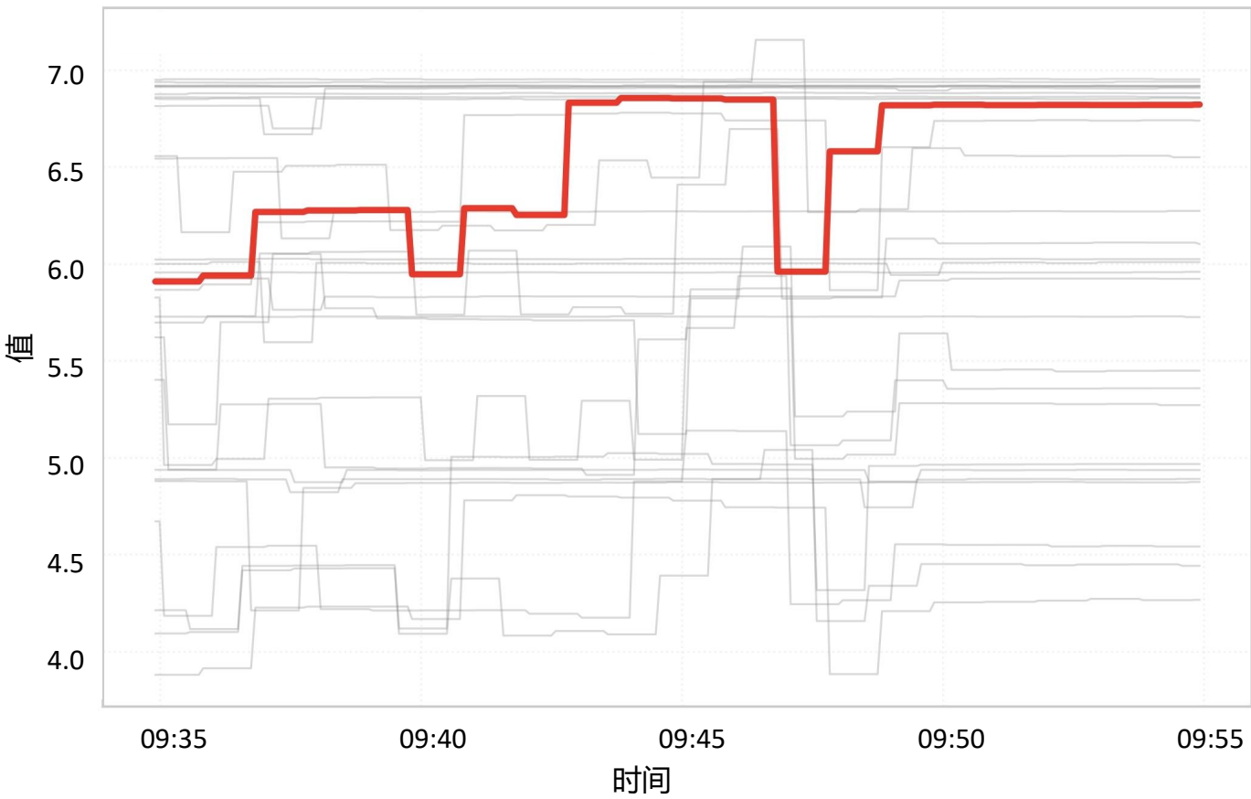
mem_usage
