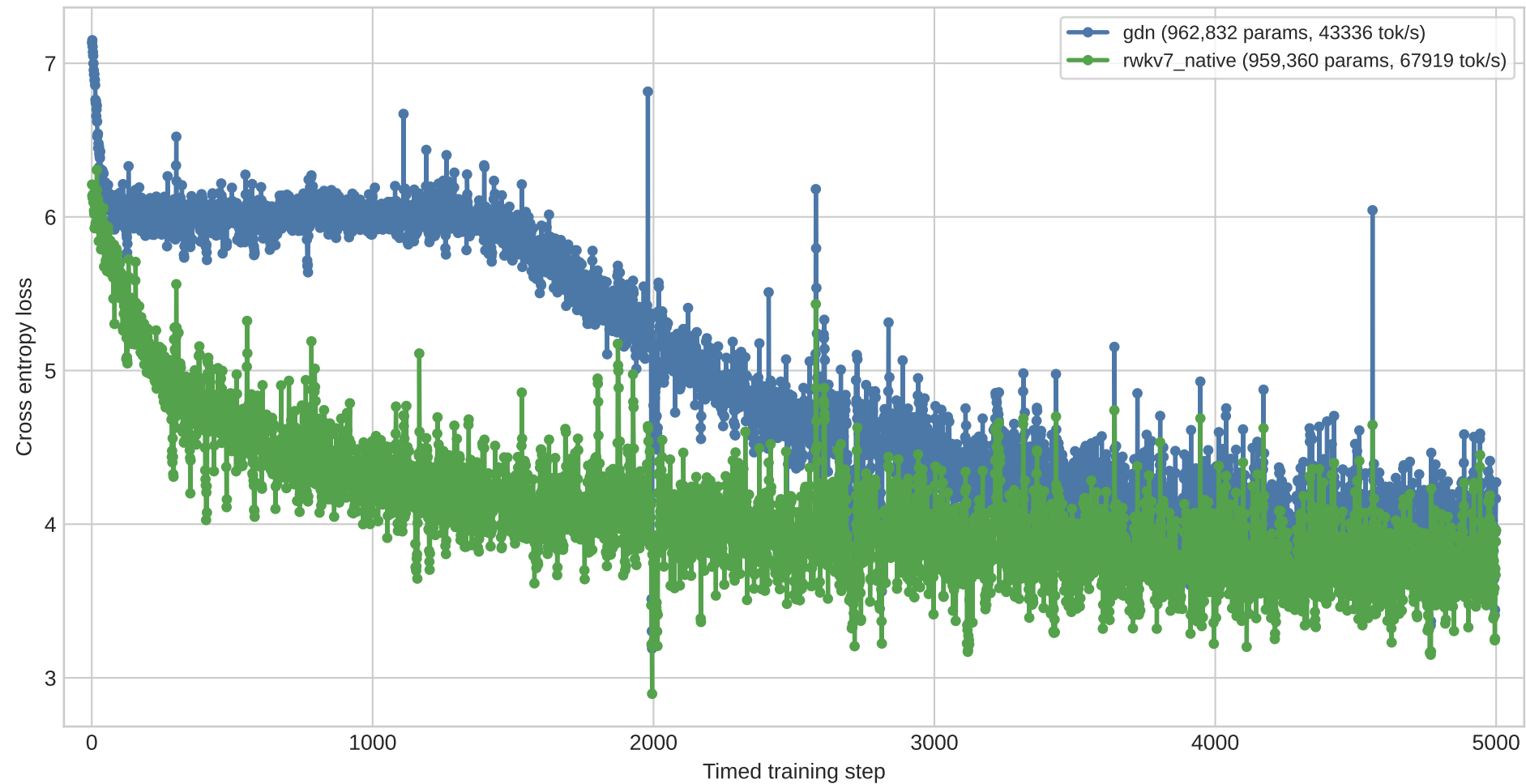
Full RWKV-7 Native vs GDN (FineWeb sp1024, 5000 steps)
