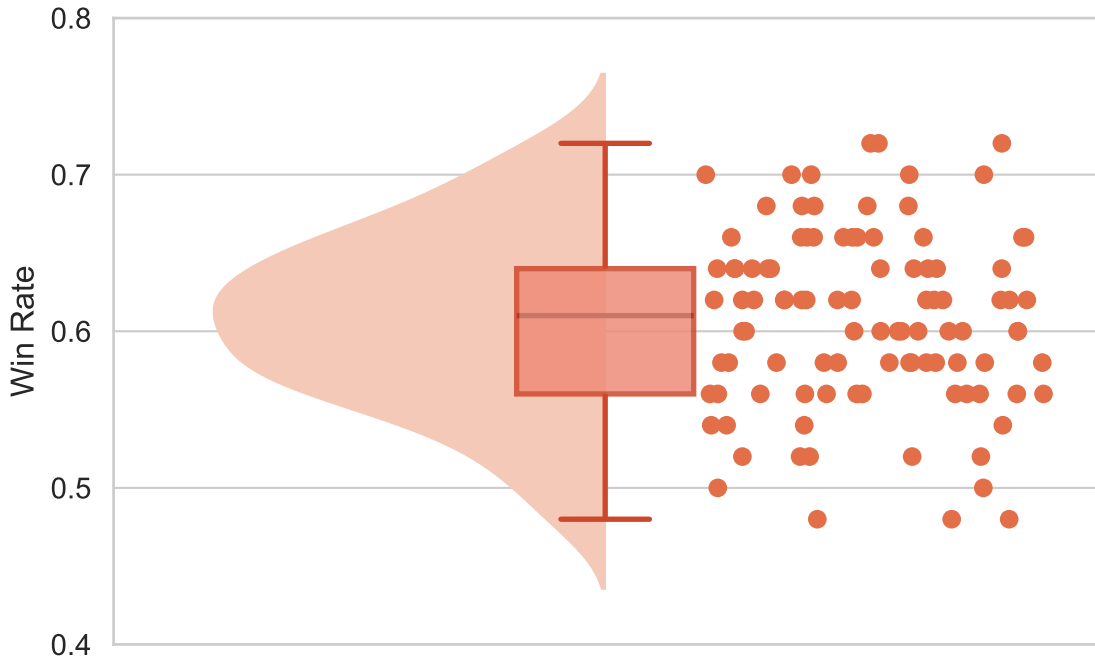
Win Rate Distribution over 100 Evaluation Rounds
