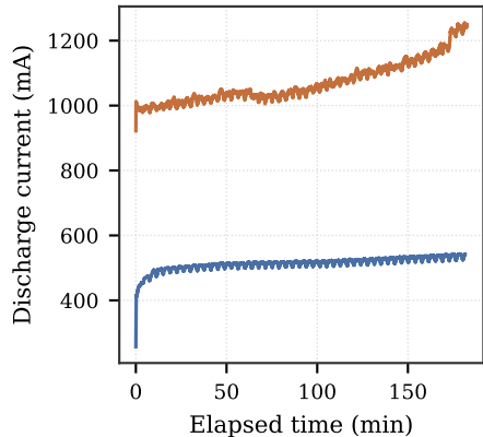
(c) Pack-side current
