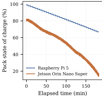
(a) Pack discharge
