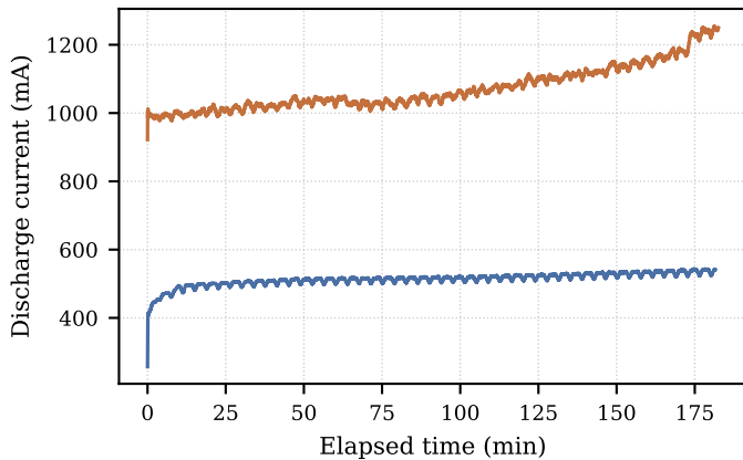
(c) Pack-side current (60-sample mean)
