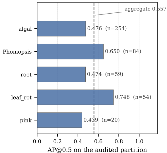
Leaf model (YOLOv11s)
