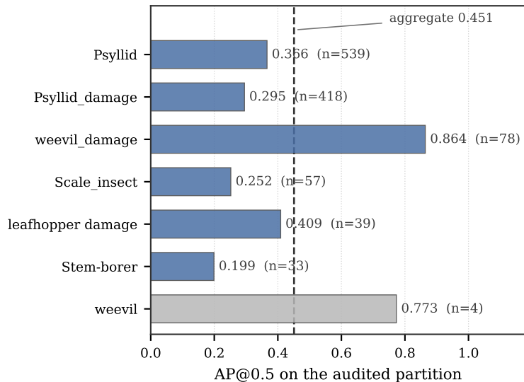
Pest model (YOLOv11n)
