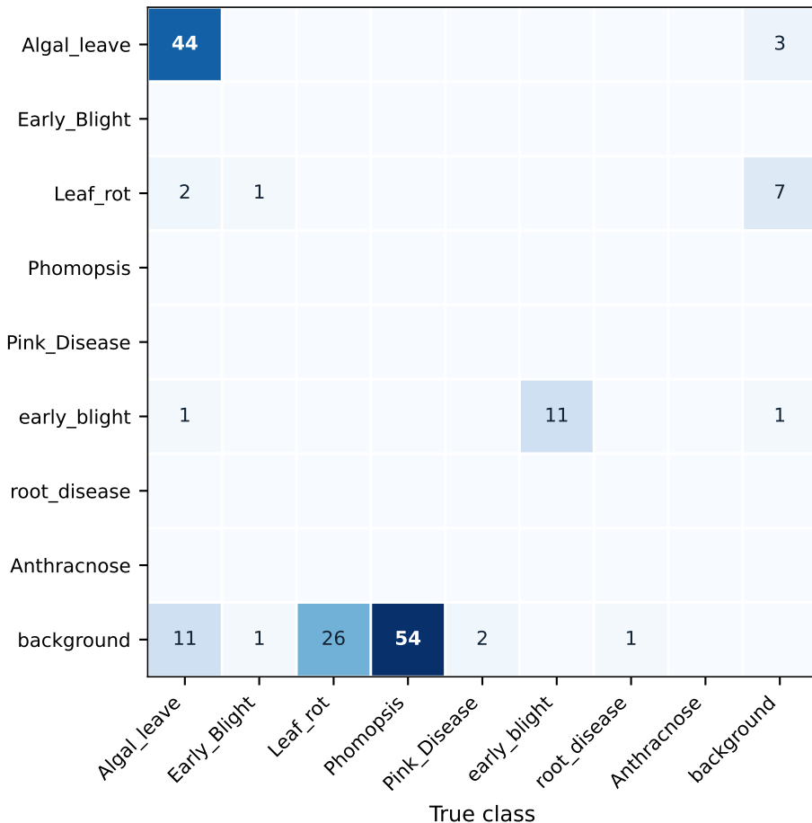
Confusion matrix, YOLOv8s under the pre-cleanup eight-class taxonomy
