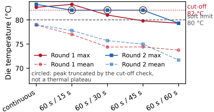
Peak temperature against the two limits
