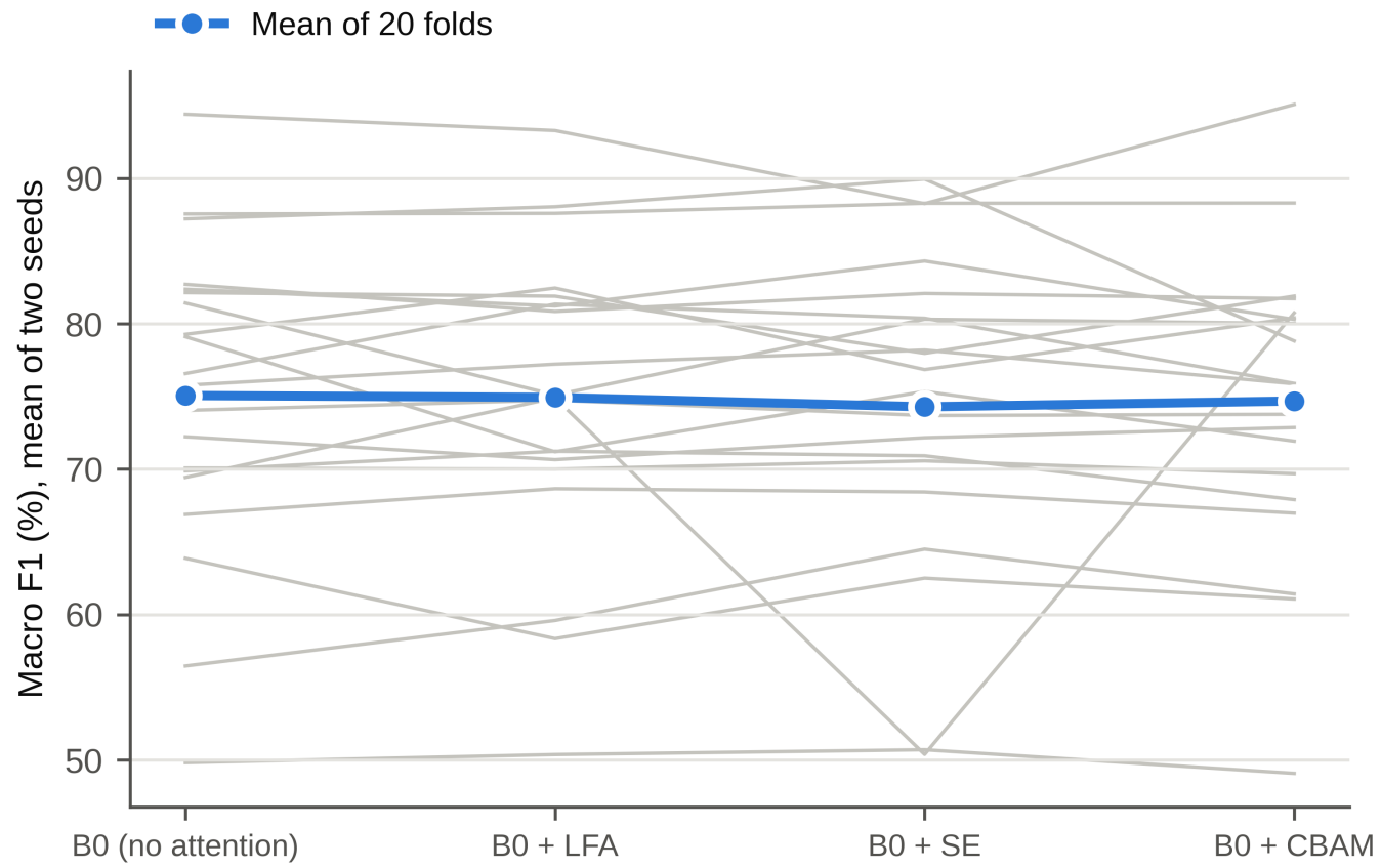
Figure S2: Macro F1 of each configuration on each of the 20 folds (grey lines, mean of two seeds) and the mean over folds (blue), all test images.
