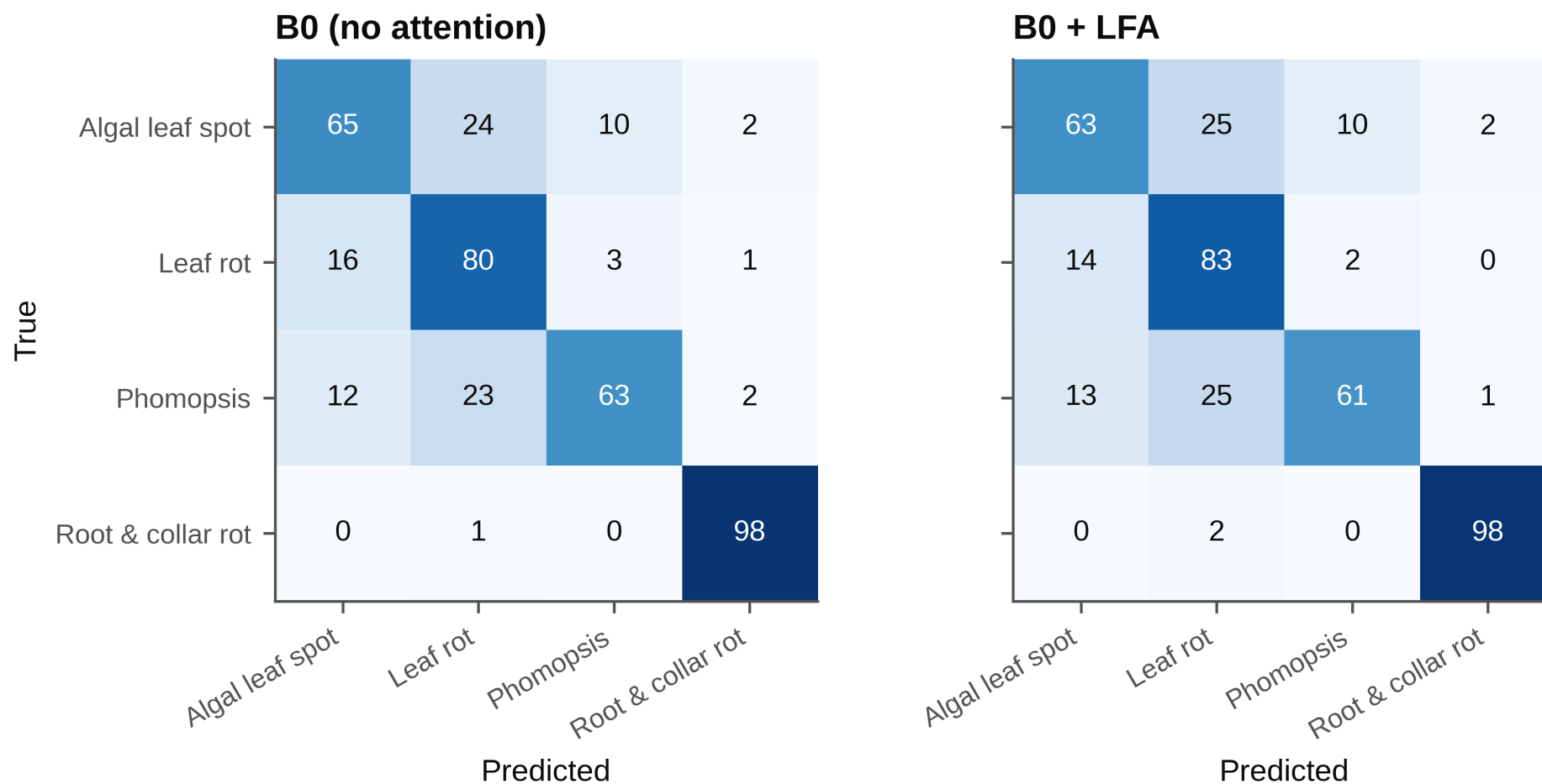
Figure S1: Confusion matrices of the plain network and the SG (labelled LFA), pooled over the 40 runs of each configuration and normalised by row (%), all test images.
