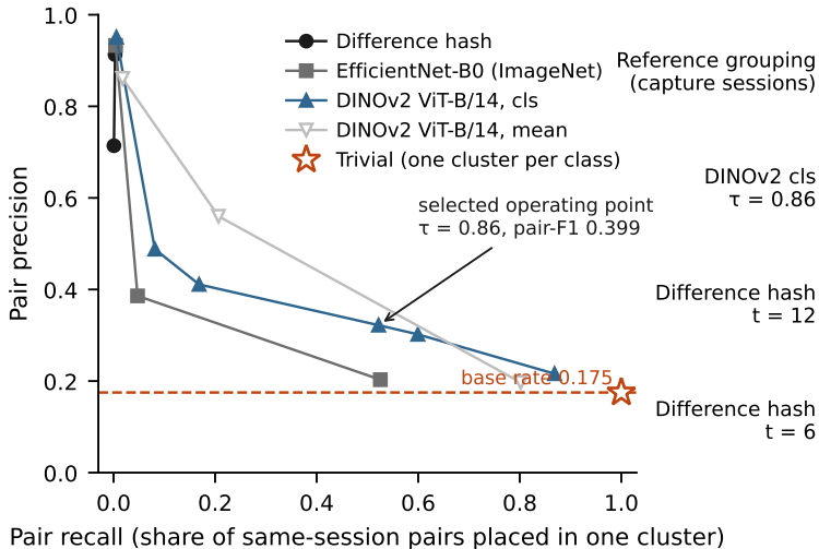
(a) Precision-recall vs the reference
