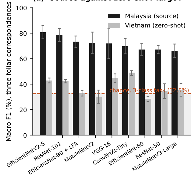
(a) Source against zero-shot target
