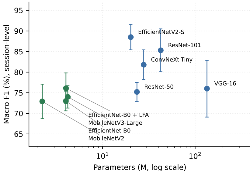
Accuracy against capacity
