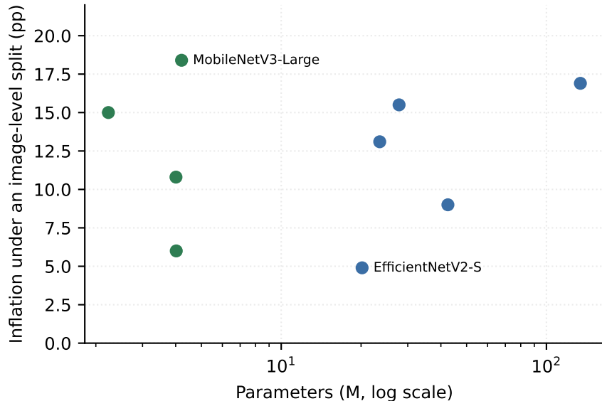
Capacity does not predict susceptibility (Pearson r = 0.29 , p = 0.45 )
