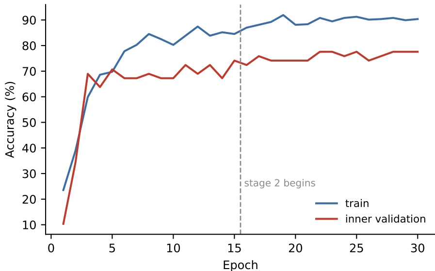
EfficientNet-B0 + LFA, comparison instance, seed 42
