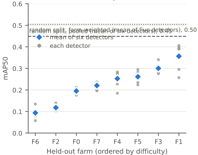
a Each farm, scored by models that never saw it
