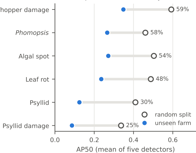
b AP kept on a new farm, by class
