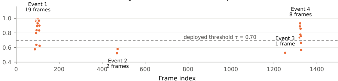
(b) The four intrusion events, all assigned to Disease, none to Healthy
