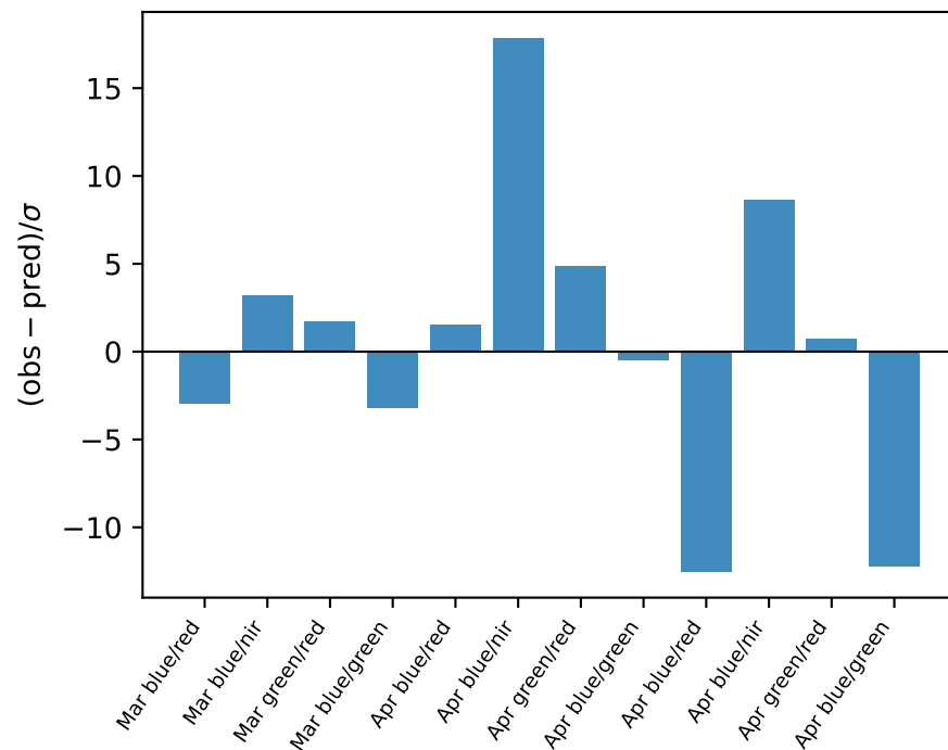
(d) Continuum shape: observed vs. reddened template
