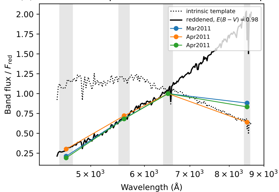
(d) Continuum shape: observed vs. reddened template
