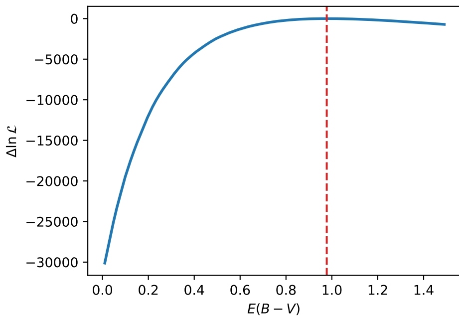
(c) Profile likelihood ( R_V = 4.8 )
