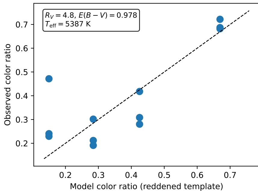
(a) Observed vs. model color ratios
