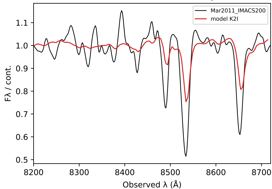
(c) Ca II + Paschen line shape
