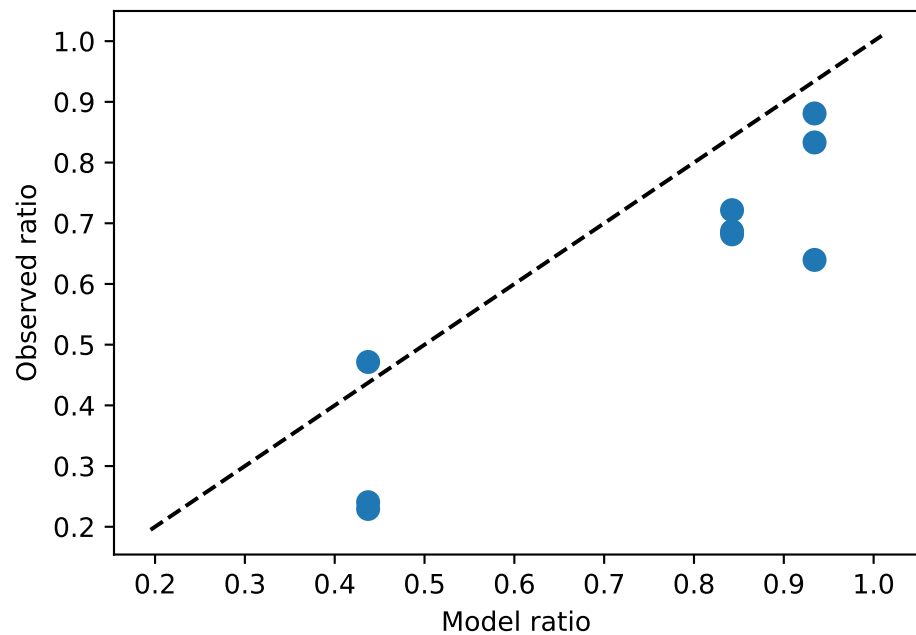
(a) Continuum color ratios
