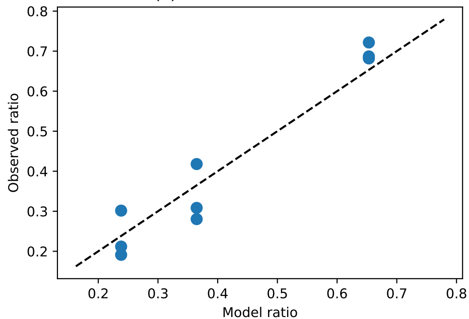
(a) Continuum color ratios
