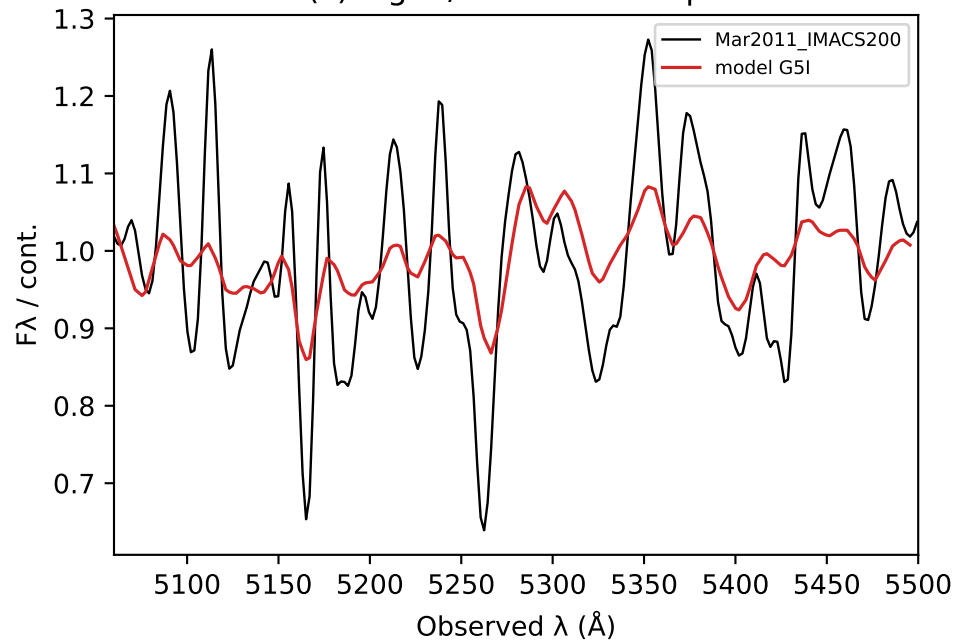
(c) Mg b / 5270 line shape
