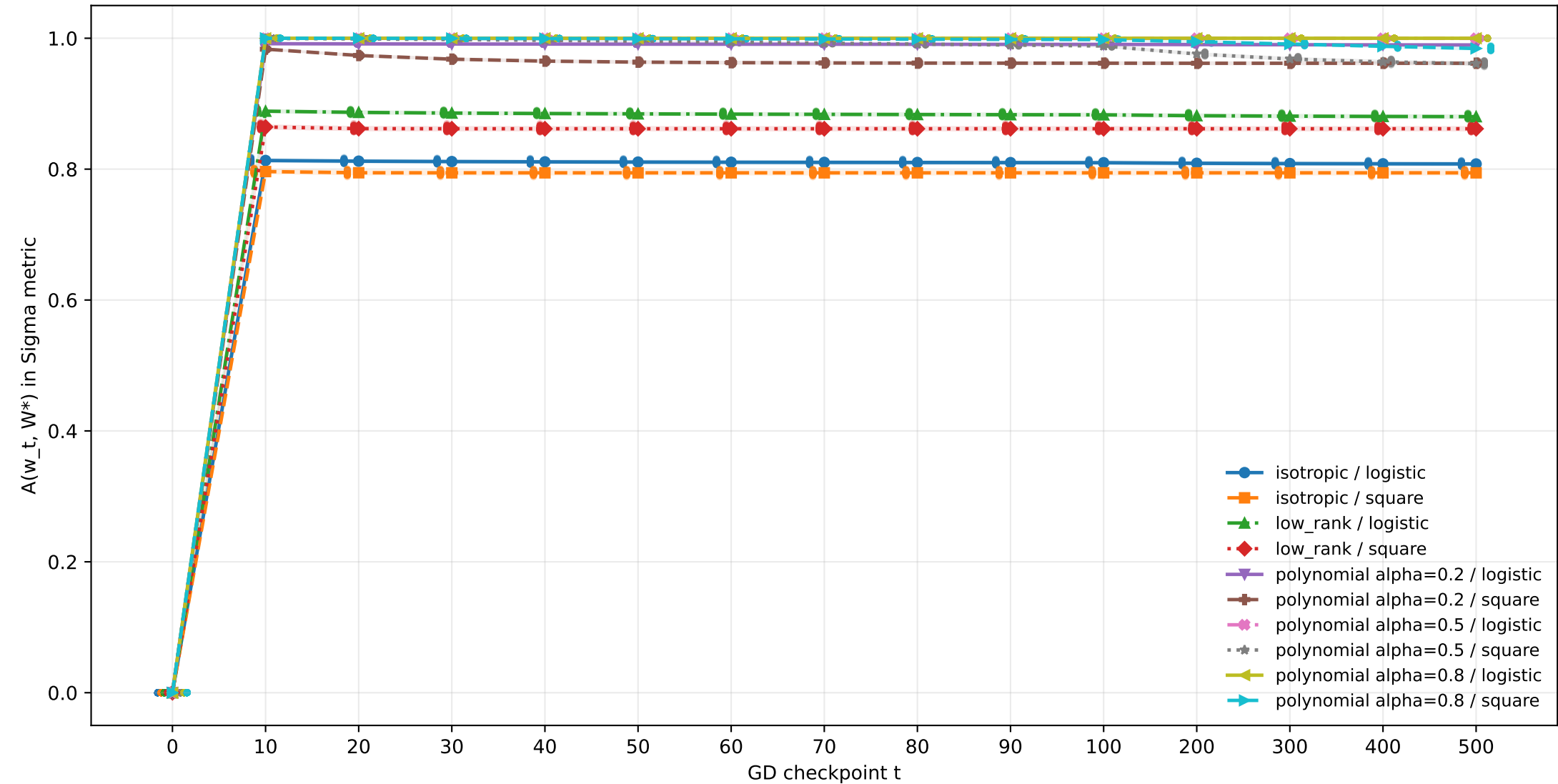
Loss baseline comparison, not theorem verification: d=20000 , n=1000 , \|\mu\|_2=6.294 , \mu \parallel v_{\max}(\Sigma)
