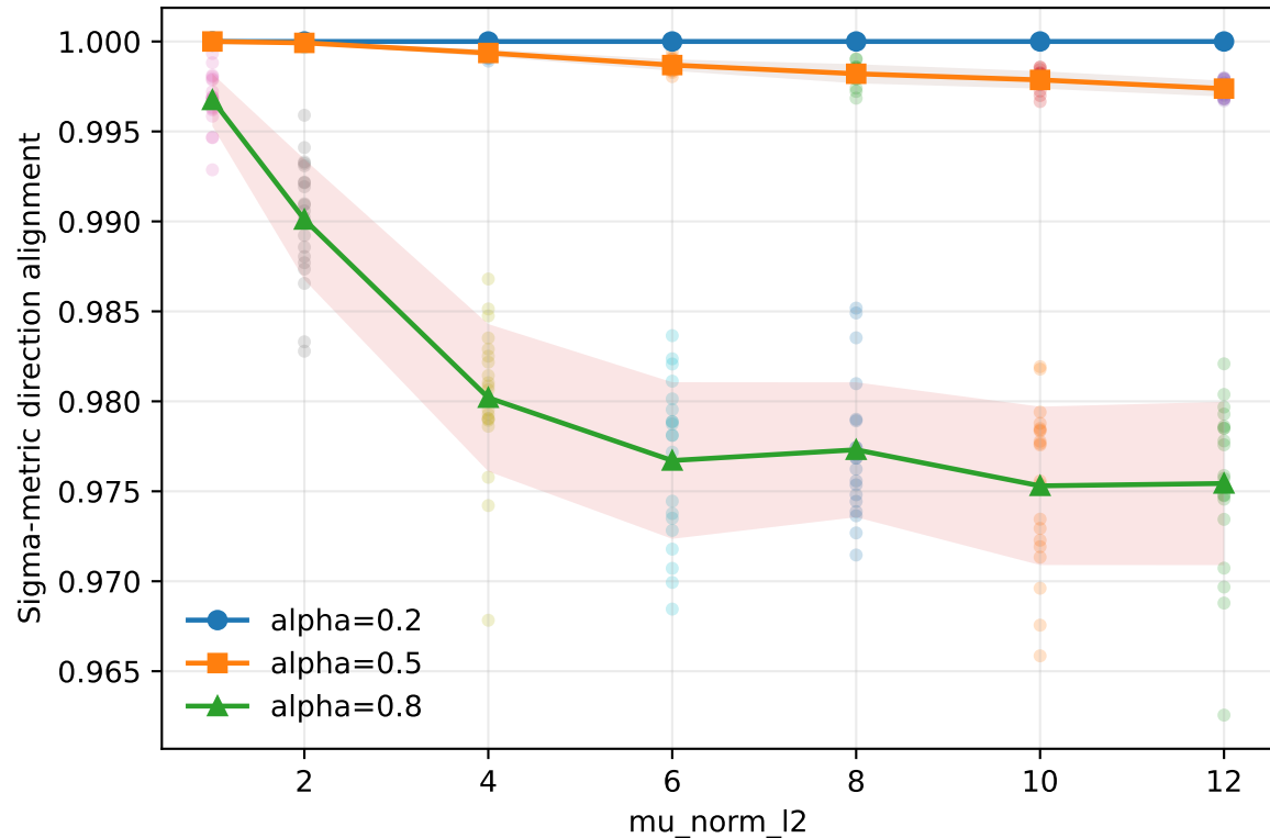
Signal threshold: A(\text{SVM}, \text{LS}) vs \|\mu\|_2
