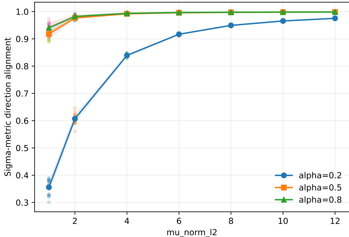
Signal threshold: A(\text{SVM}, W^*) vs \|\mu\|_2
