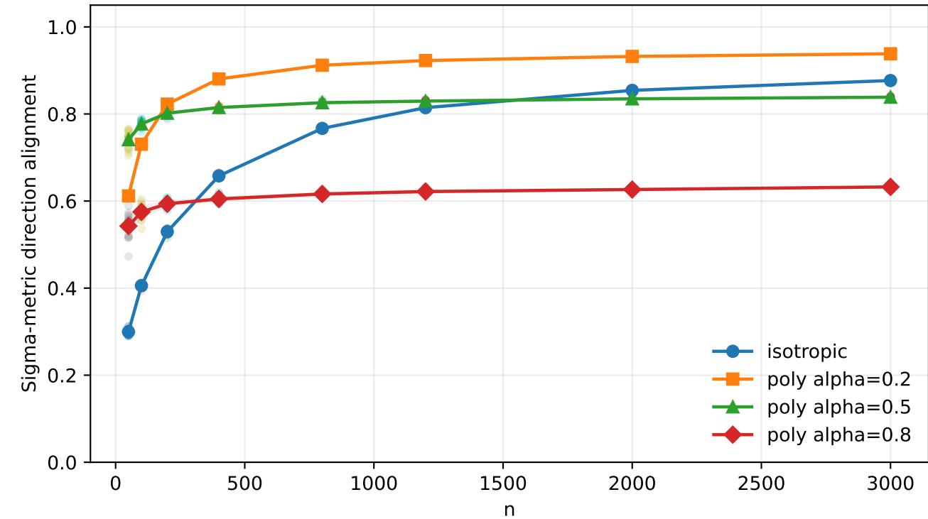
Fixed d=20000 : A(\text{SVM}, W^*) vs n
