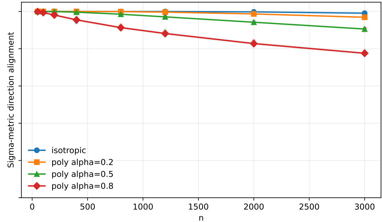
Fixed d=20000 : A(\text{SVM}, \text{LS}) vs n
