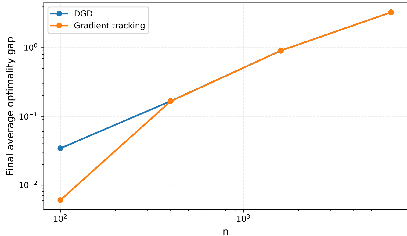
Dependence on the dataset size
