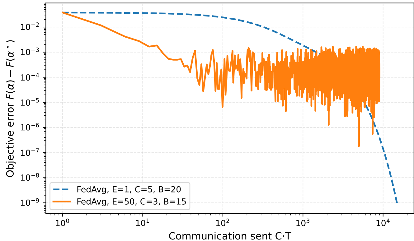
FedAvg under a communication budget
