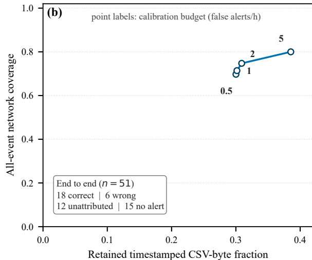
Coverage--retention frontier
