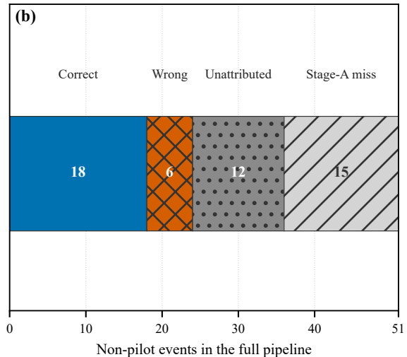
Final outcomes expose abstention and misses
