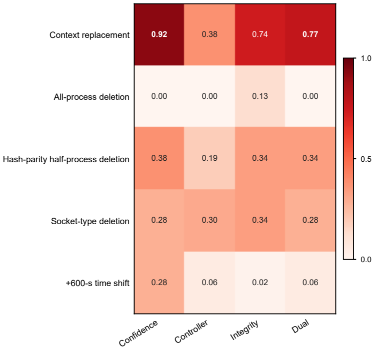
Wrong-label rate
