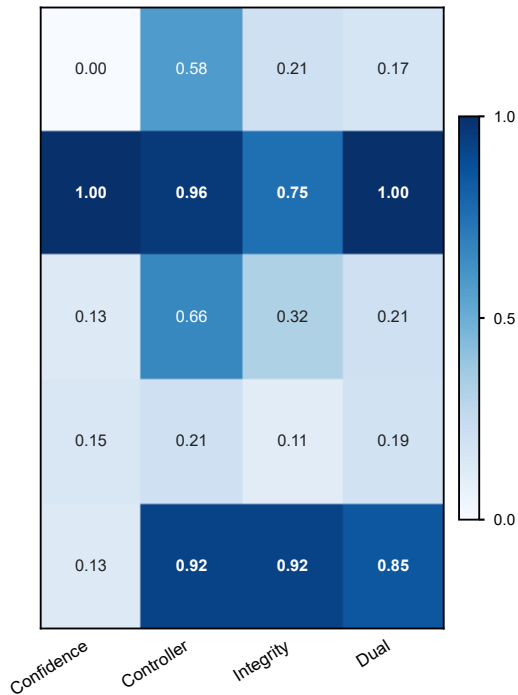
Rejection rate
