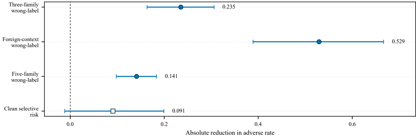
CICAPT-IIoT: adverse-rate reduction over matched margin
