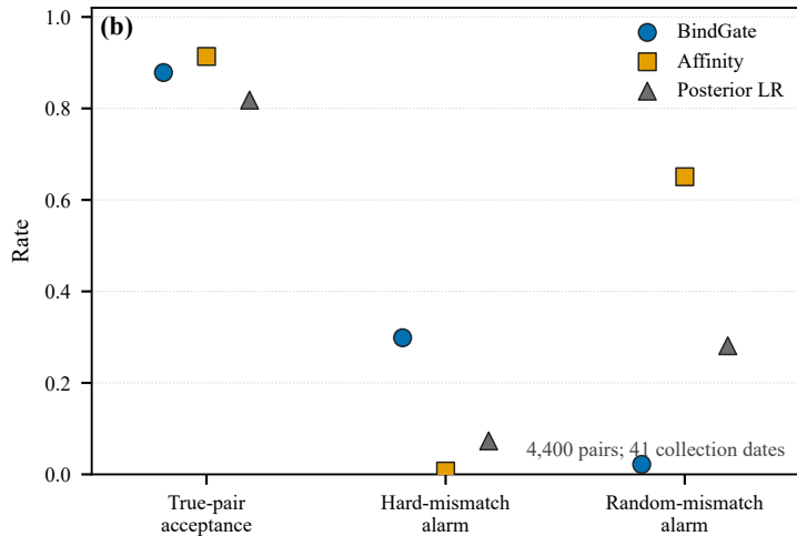
X-IIoTID: behavior depends on mismatch regime
