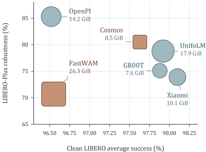
(a) Clean Capability vs. Robustness
