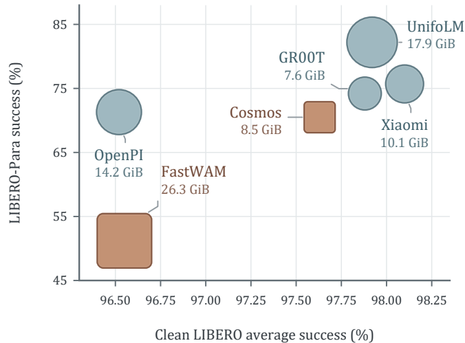
(b) Clean Capability vs. Language Sensitivity
