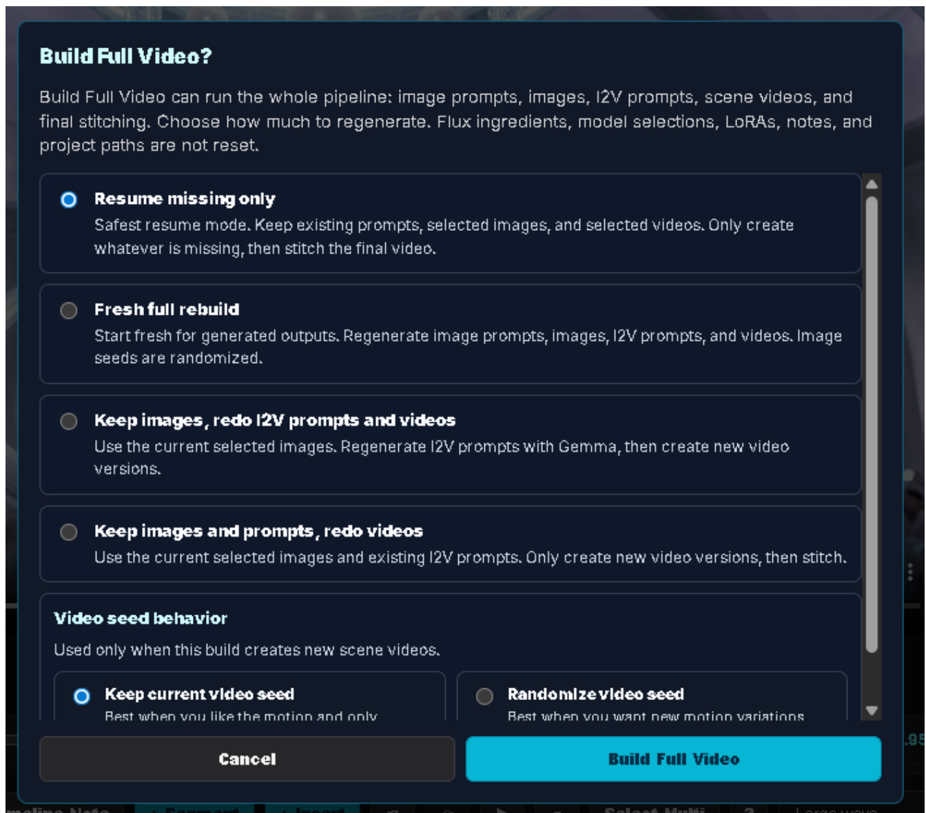
Build Full Video Options
