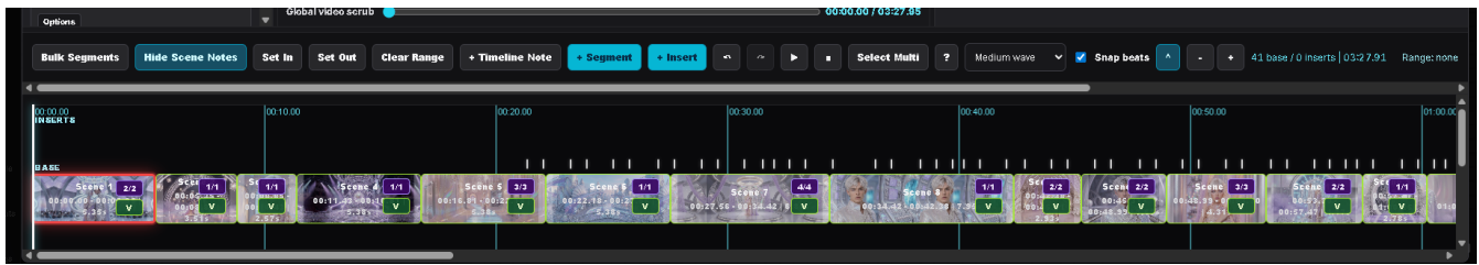
Timeline Controls
