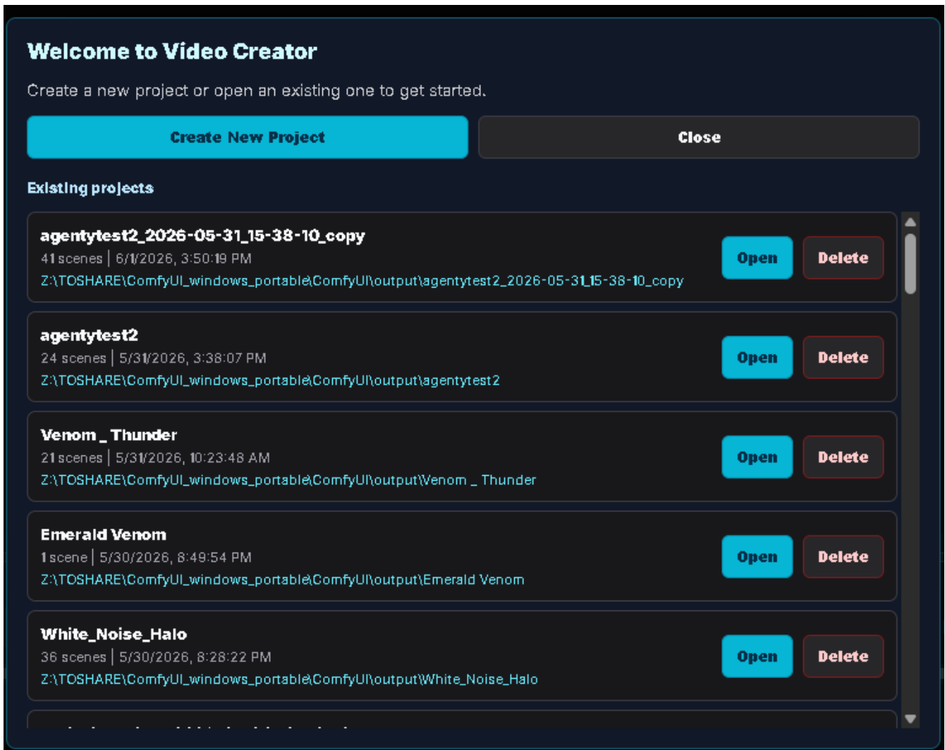
Welcome Window
