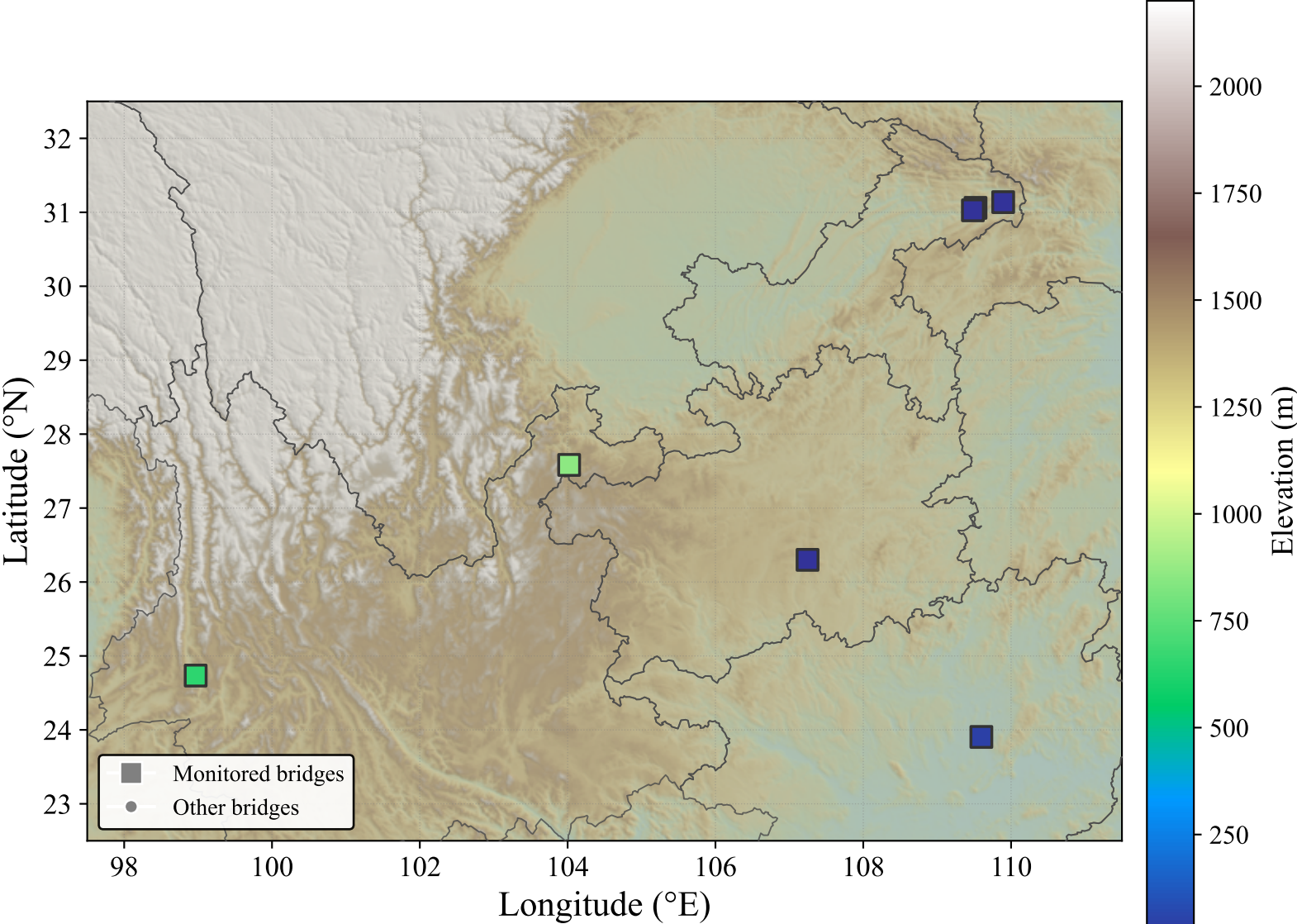
(a) DEM of the study area (ETOPO1 1 km shaded relief; dots = bridges coloured by GLO-90 elevation)
