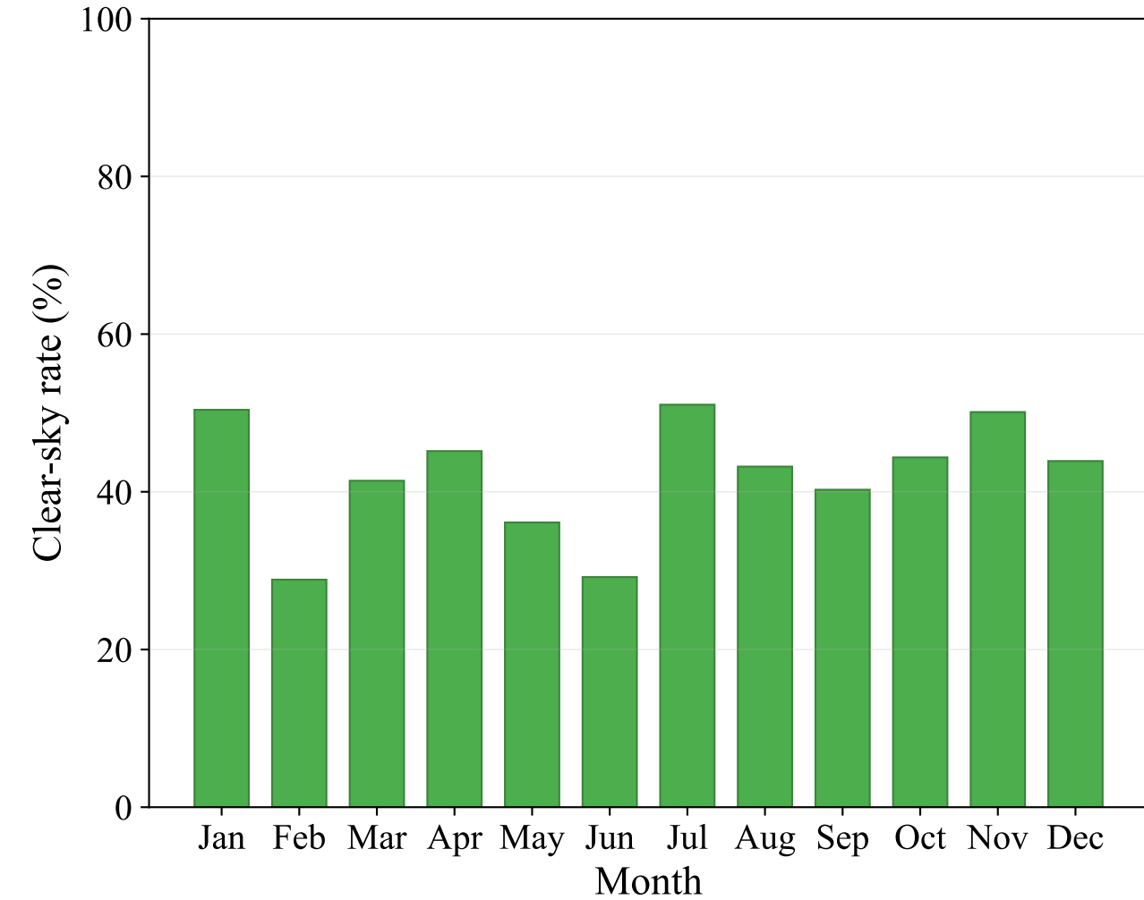
(c) Monthly daytime clear-sky rate
