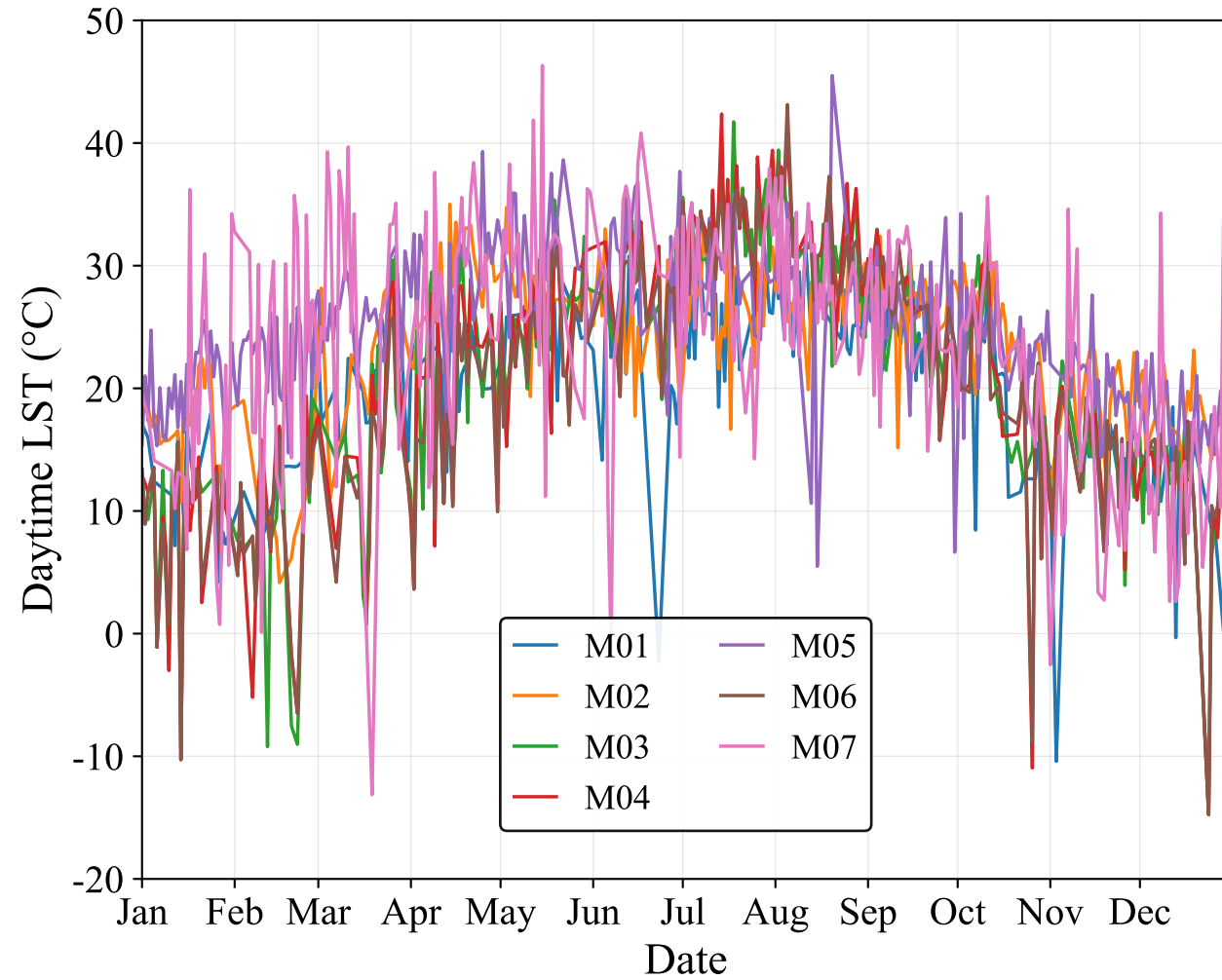
(a) Daily daytime LST of the 7 monitored bridges
