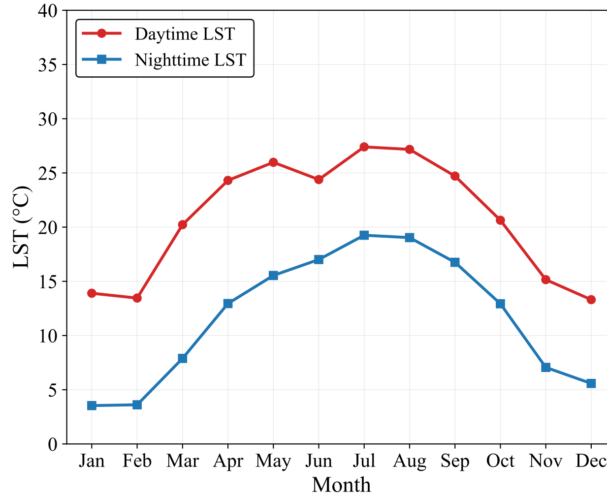
(b) Annual cycle of monthly mean LST (207 bridges)
