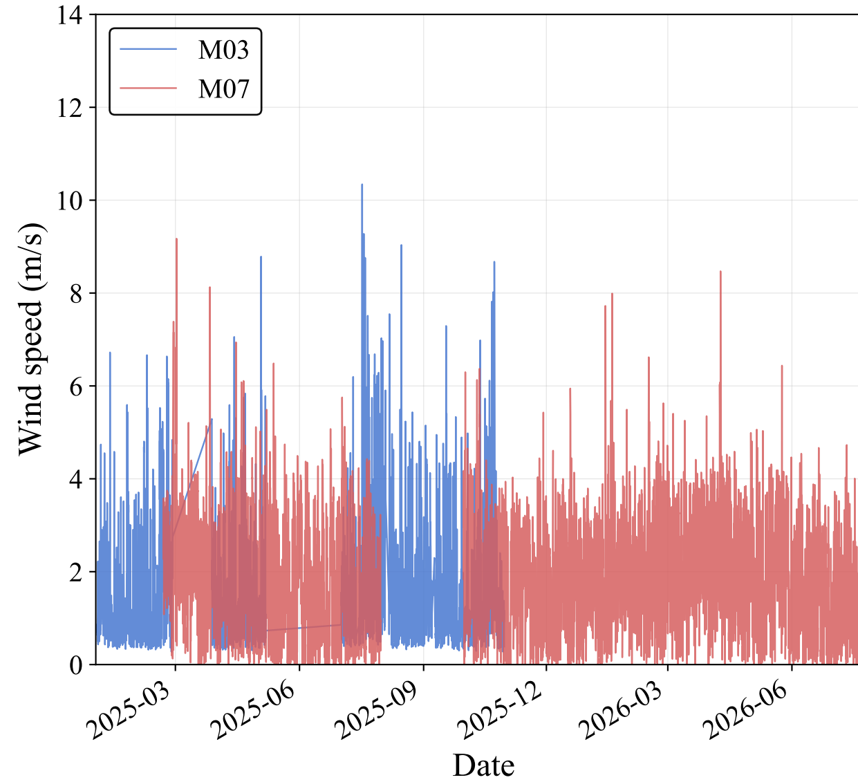
(b) Hourly wind speed at M03 and M07
