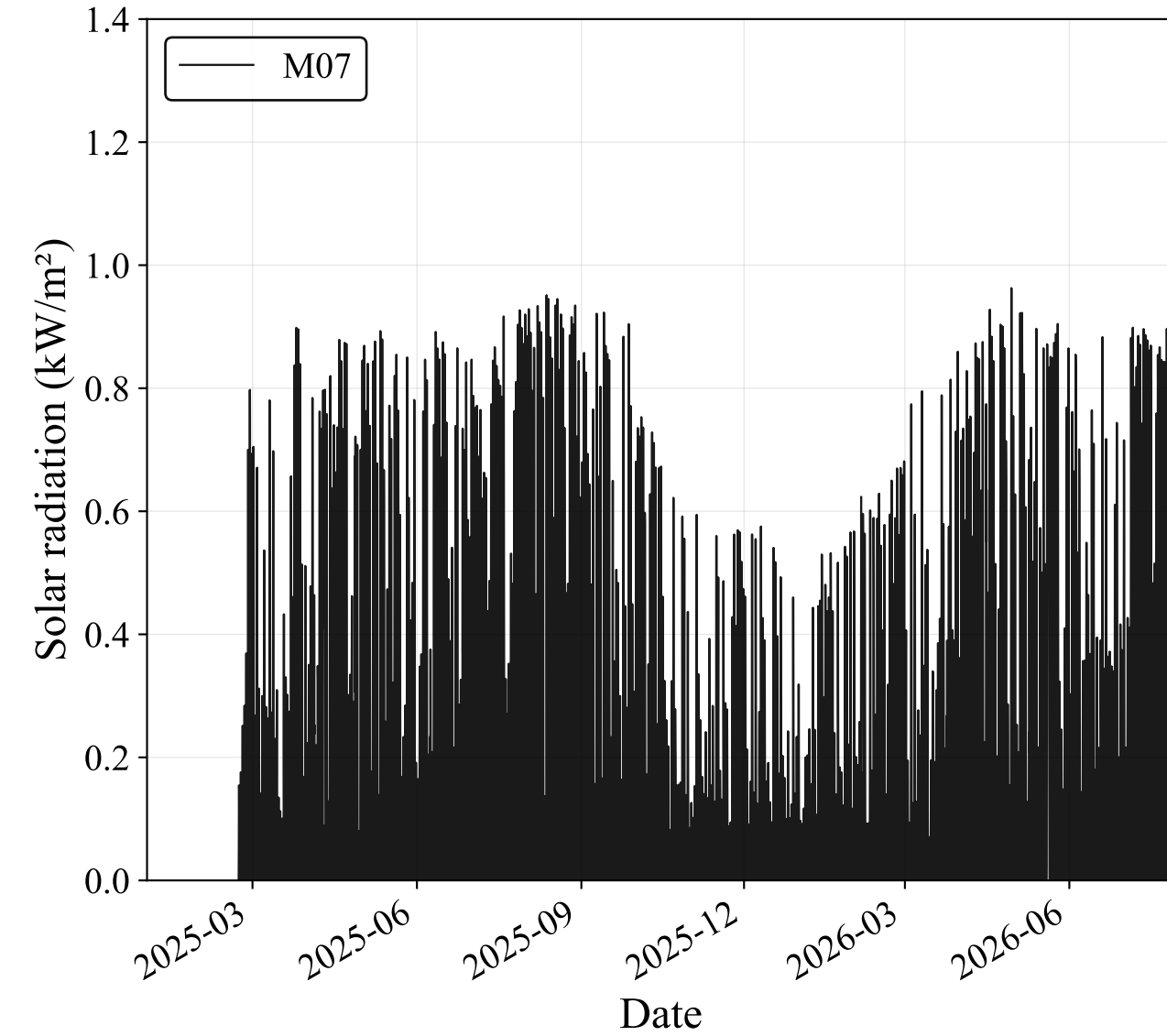
(c) Hourly solar radiation at M07
