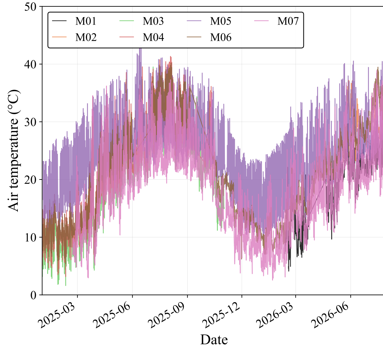
(a) Hourly air temperature of the 7 monitored bridges (M01 since Feb 2026, M02 since May 2026)
